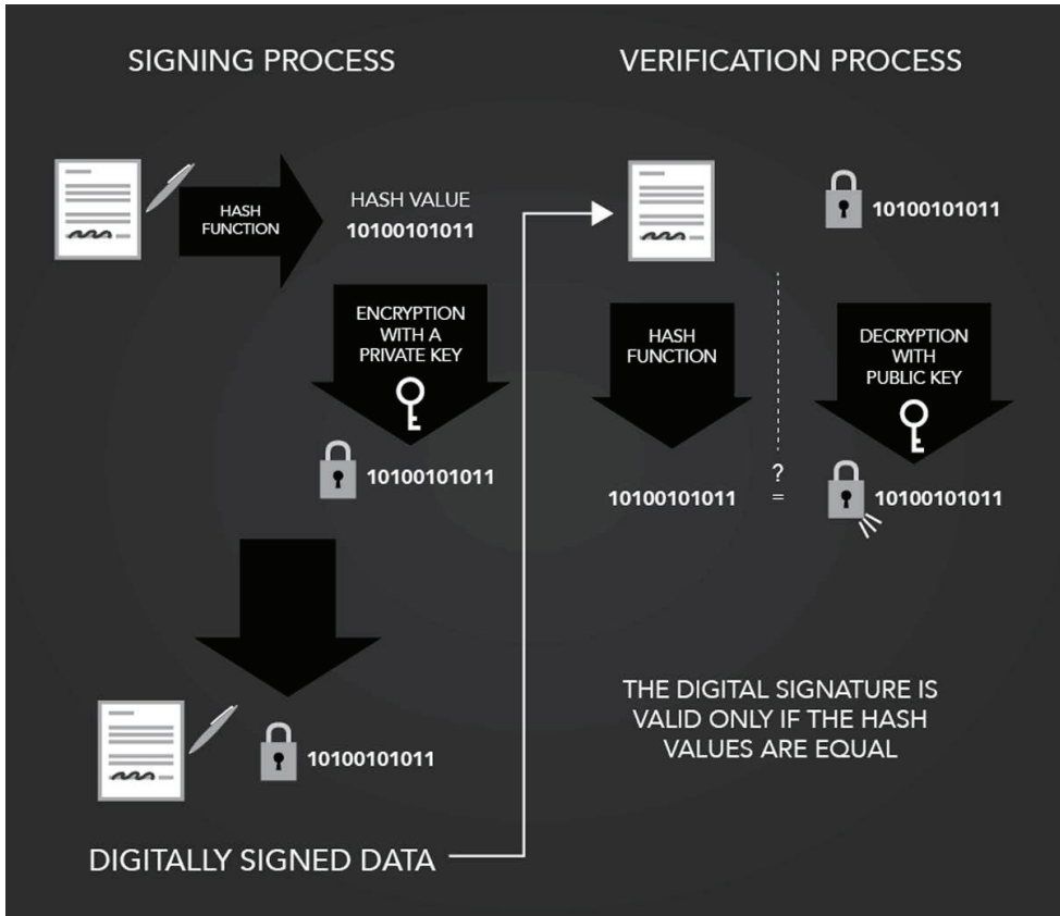
Figure 8 Digital Signatures - How it works
